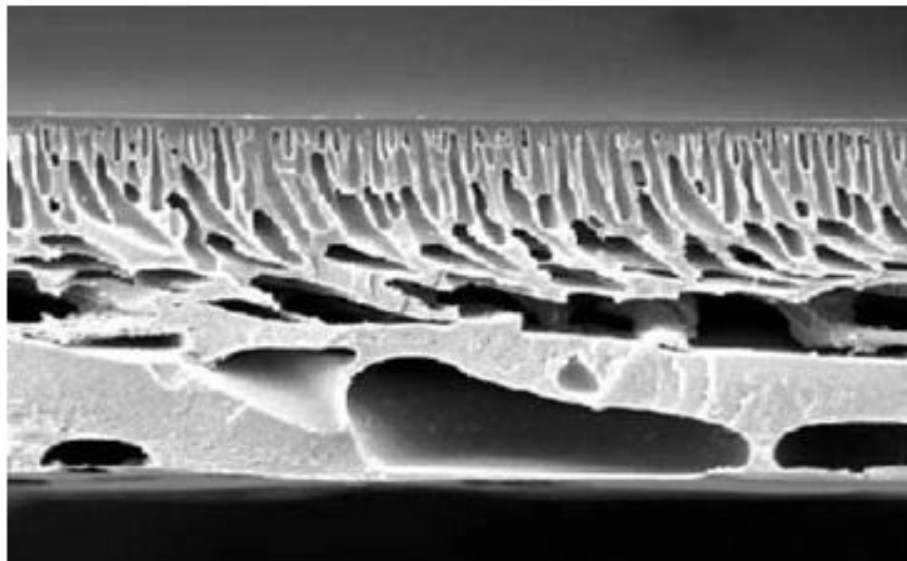
Fig. 2 Skin layer structure of a UF membrane. (Courtesy of Sartorius AG.)
