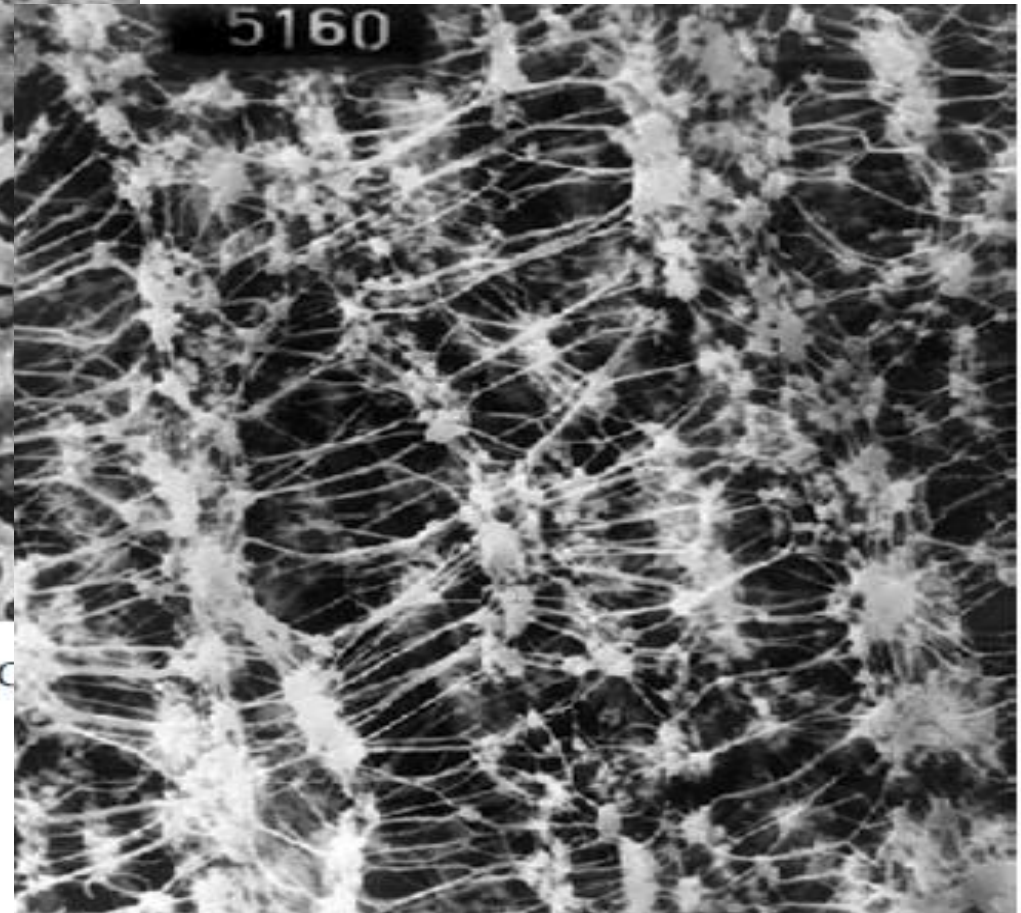
5 PTFE membrane structure. (Courtesy of Sartorius
