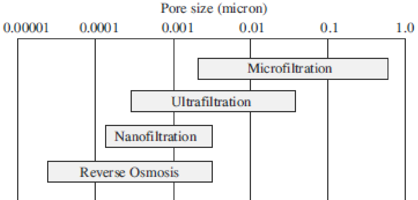
Fig. 1 Typical pore sizes for membranes used in reverse osmosis, nanofiltration, ultrafiltration, and microfiltration.
